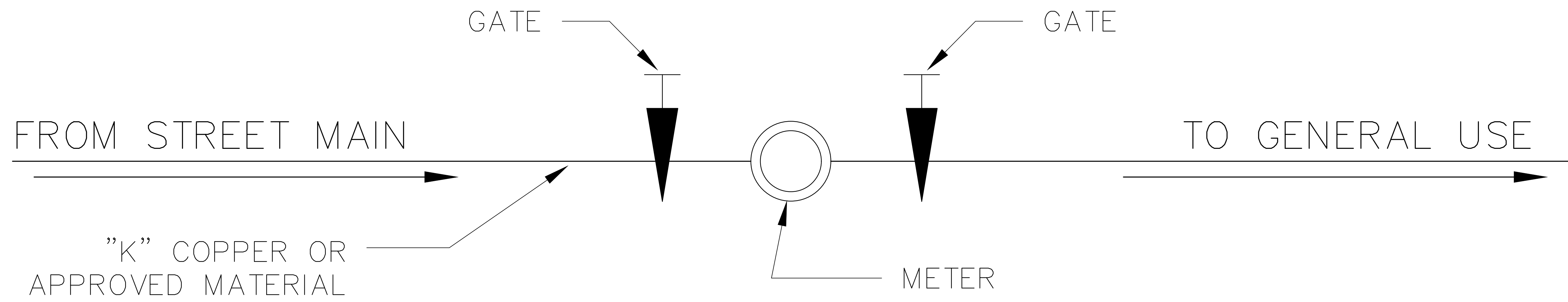
RESIDENTIAL WATER SERVICE DETAIL N.T.S.
